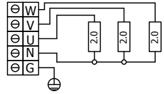
DRFT3-60NS-CNR 6,0 kW
